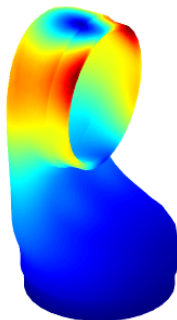
Flexible Mode 4 Frequency = 5112.6 Hz
