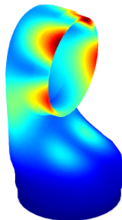
Flexible Mode 5 Frequency = 7819.53 Hz
